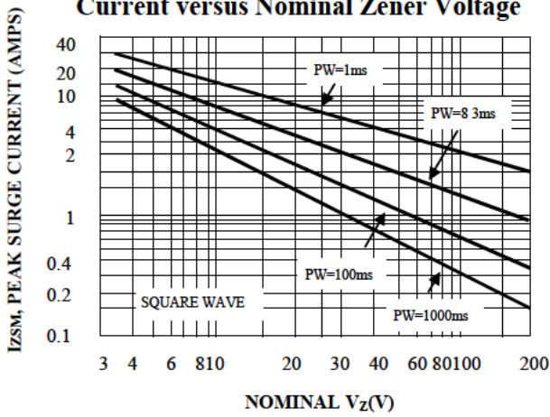
Figure 6. Maximum Non-Repetitive Surge Current versus Nominal Zener Voltage
