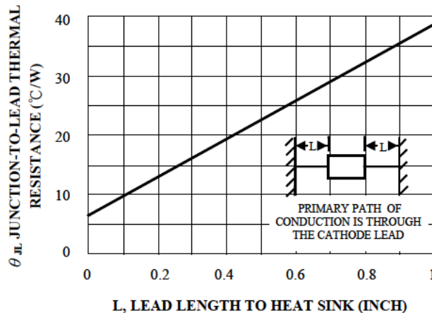
Figure 5. Typical Thermal Resistance
