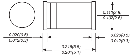
Case: MELF Dimensions in inches and (millimeters)
