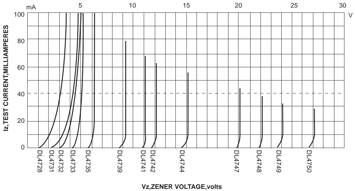
Breakdown characteristics
